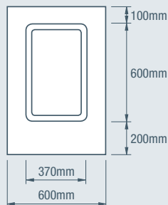
easyascot® standard panel AP900
