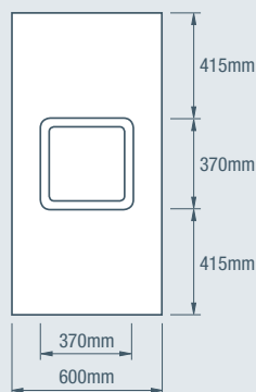
easyascot® window panel AWP1200
